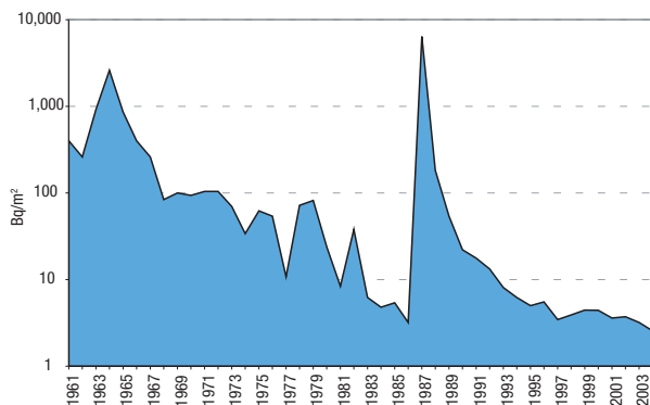
Figure 15.5: Annual trend of total fallout of Cs-137 in Italia
