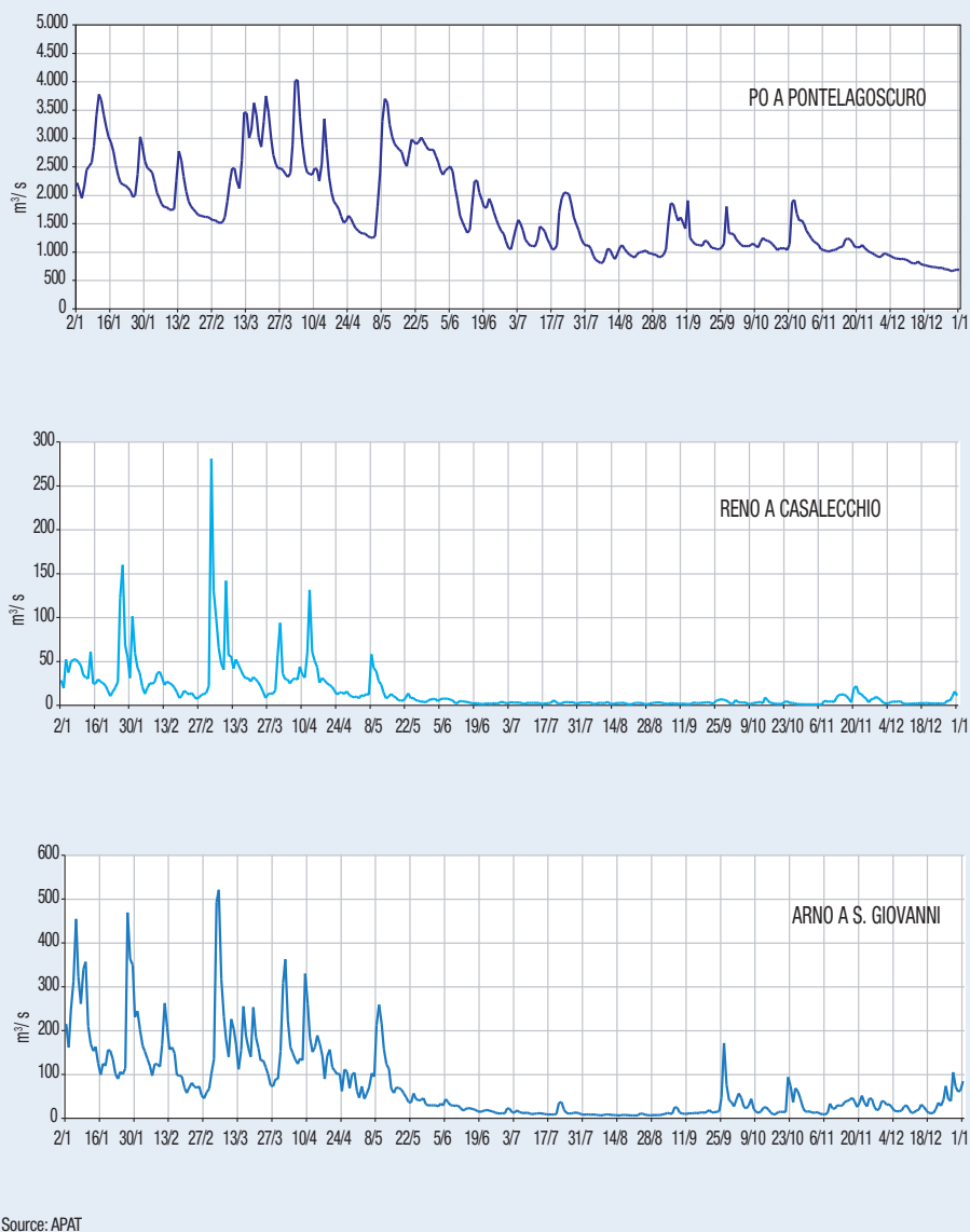
Figure 12.2: Daily outflows ( \text{m}^3/\text{sec} ) of several Italian rivers (2001)
