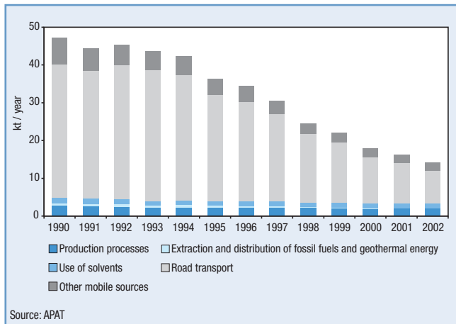
Figure 10.7: National emission of benzene (C 6 H 6 )
