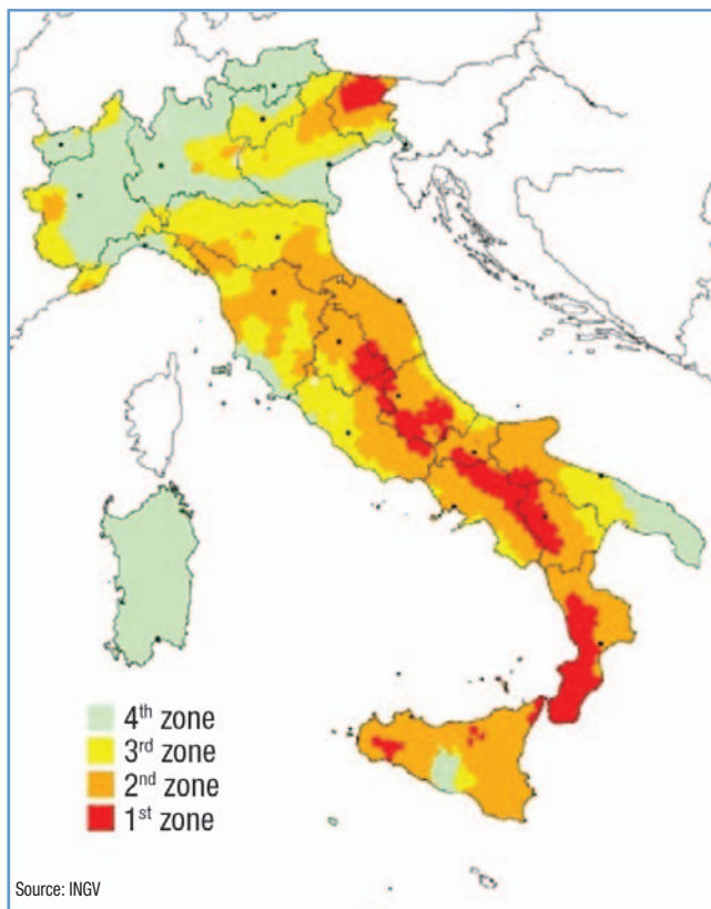
Figure 18.1: Seismic zoning map of Italy, based on the new zoning guidelines introduced in 2003, and approved in April 2004, as subsequently implemented by the regional authorities
